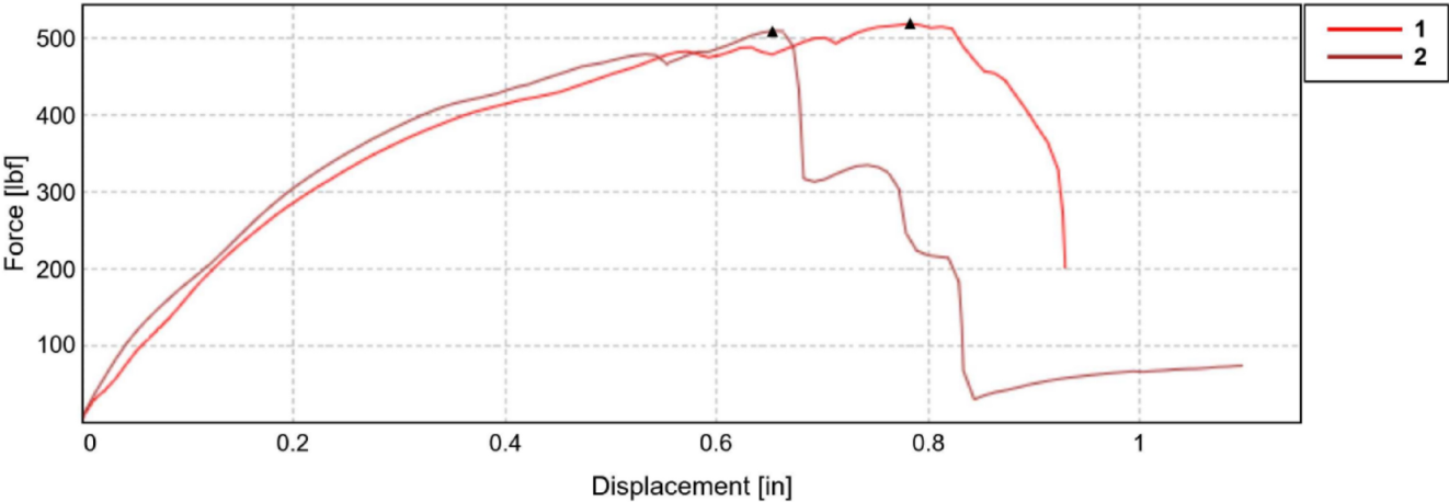
Figure 1: Tensile Force vs Displacement test graph
