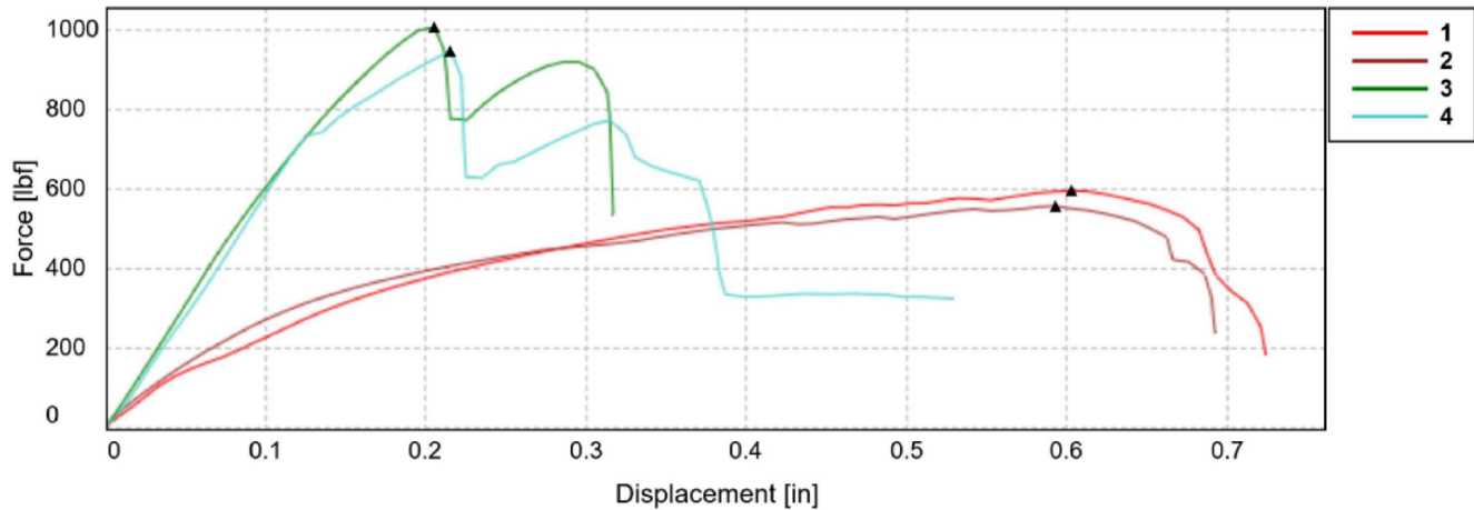
Figure 1: Tension Force vs Displacement test graph
